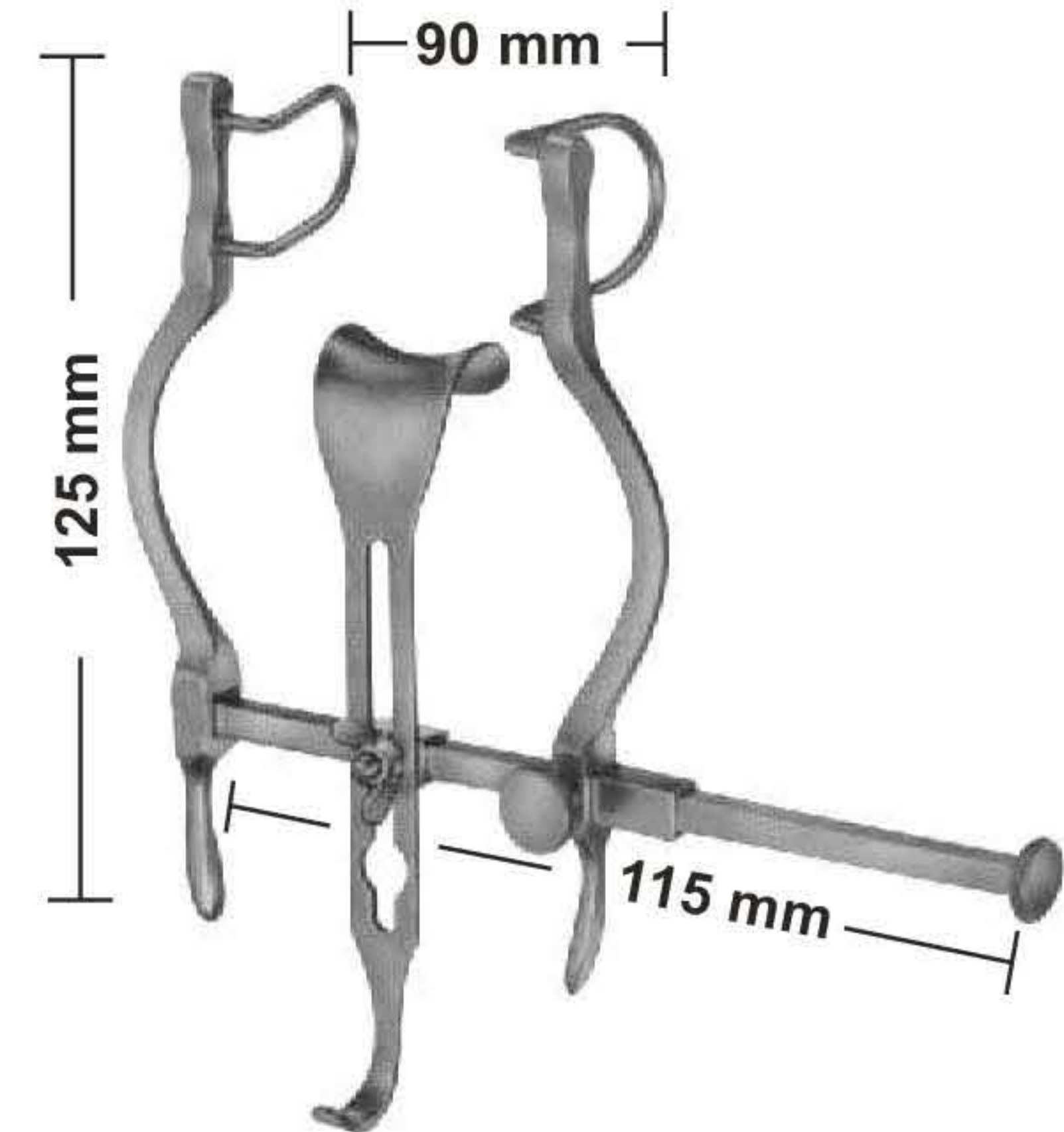
UG-1094 BALFOUR-BABY Lateral blades 27 mm deep Center blade 21x24 mm
