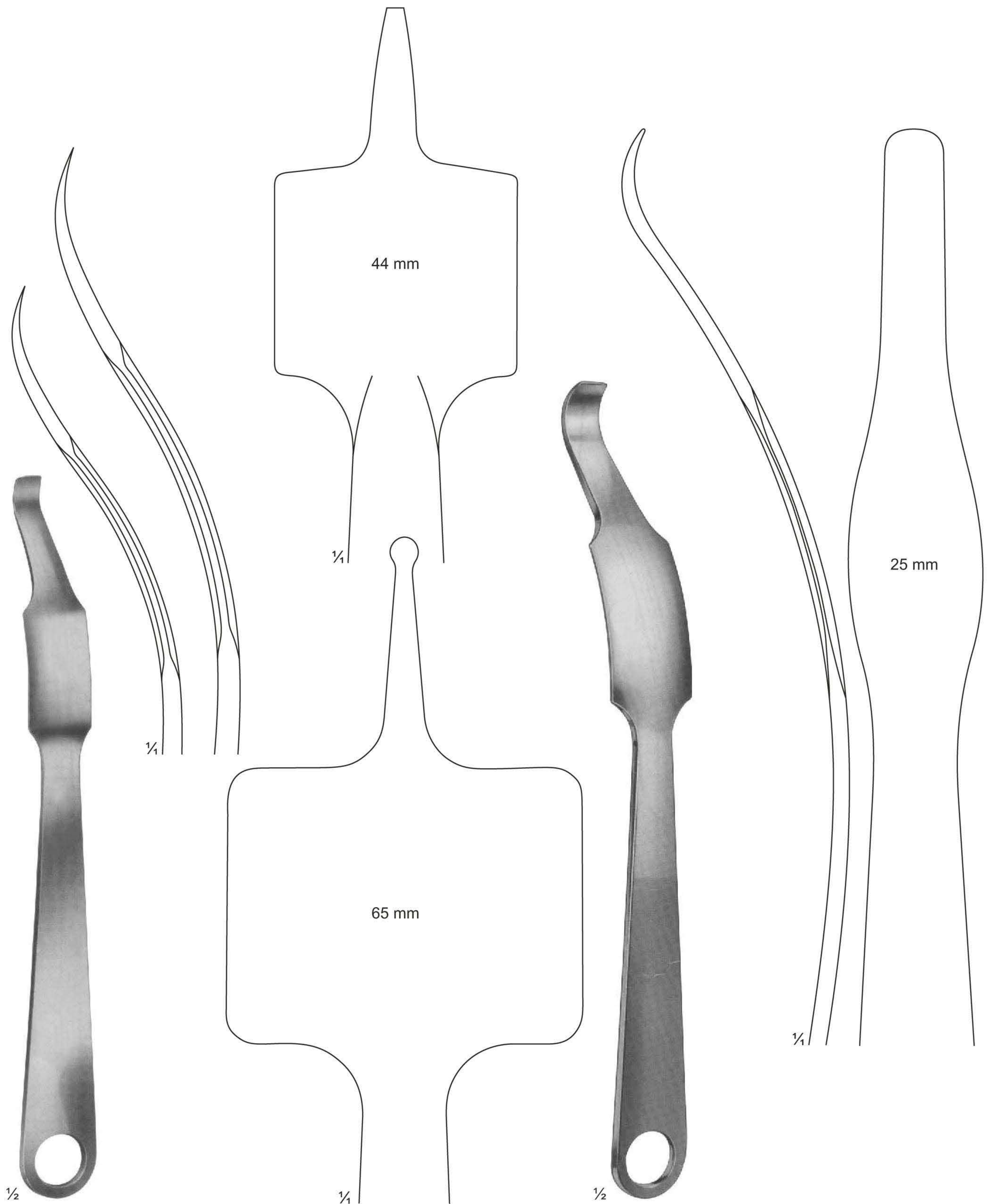
UG-1570 VERBRUGGE-MULLER UG-1571 240 mm 255 mm
