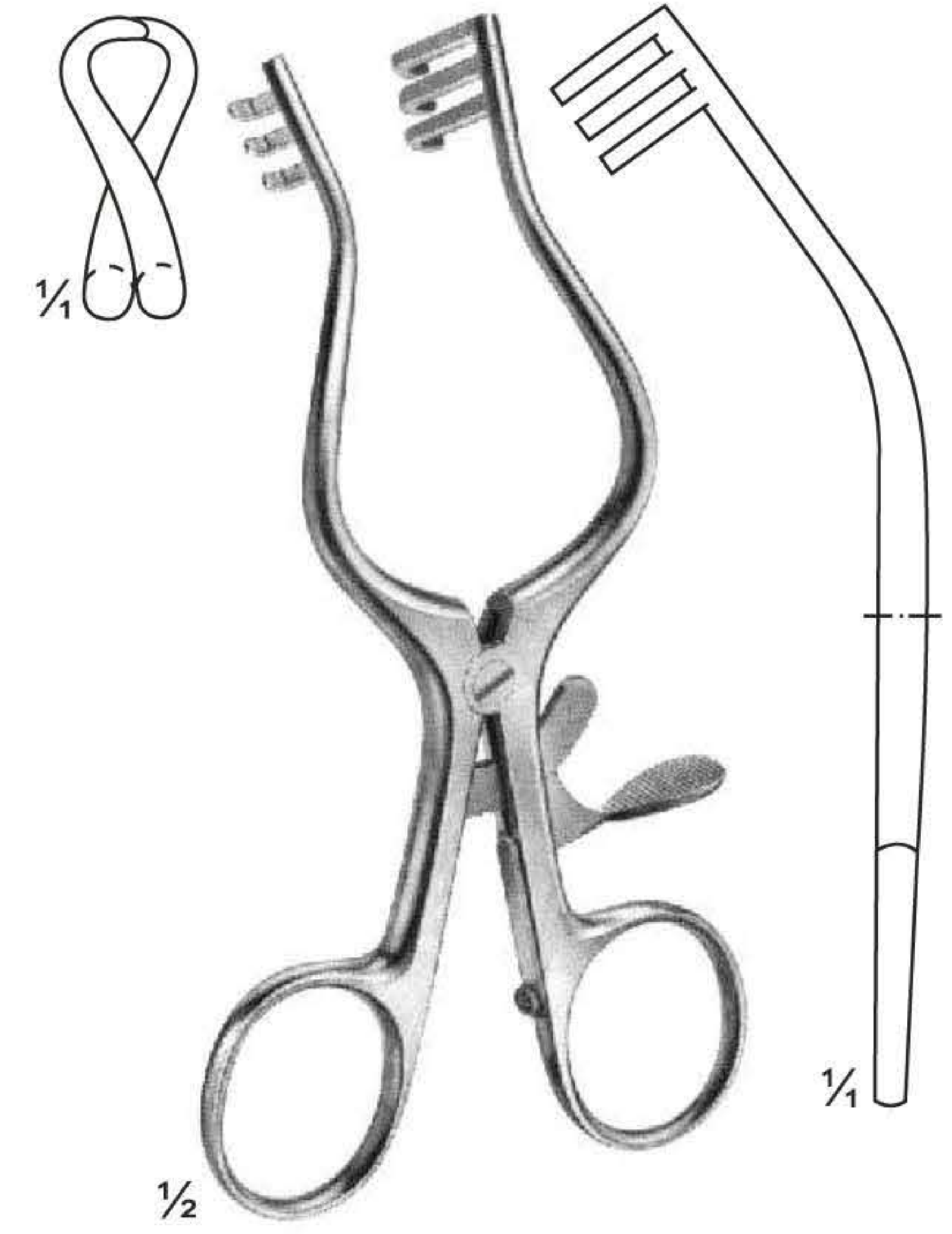
UG-1001 WULLSTEIN Blunt 130 mm
